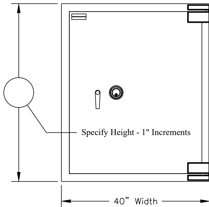
FRONT ELEVATION
